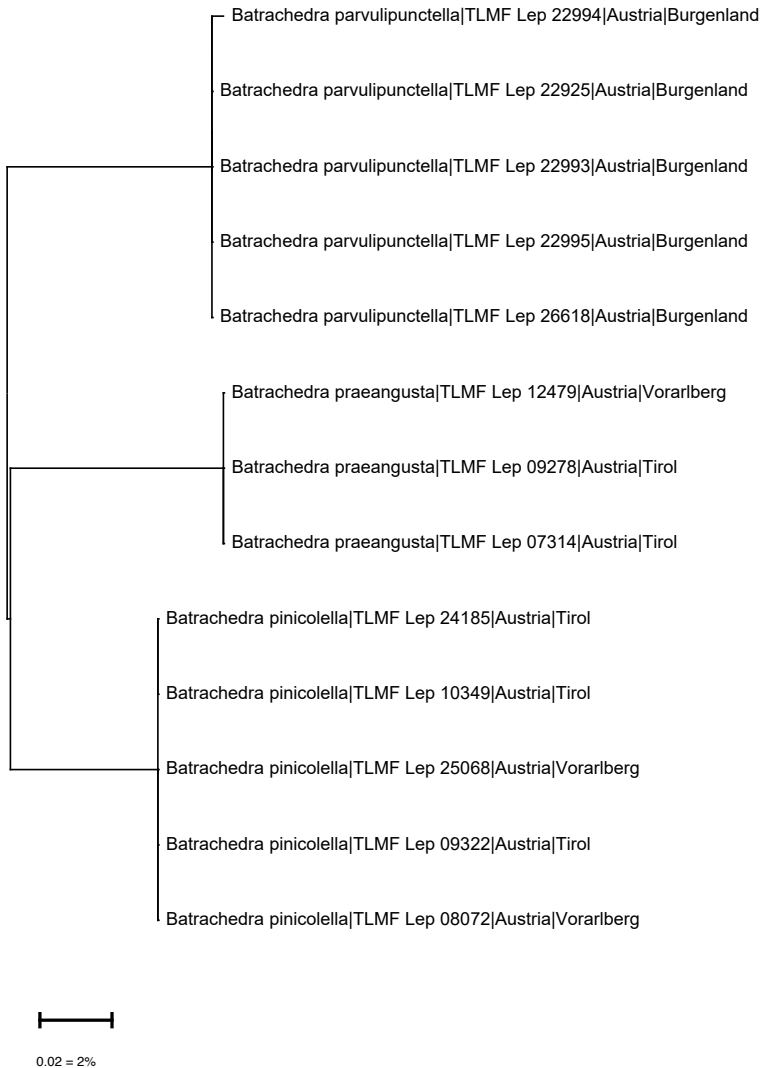
Abb. 6: Neighbour Joining tree österreichischer Batrachedra basierend auf Sequenzen des mtDNA COI-Gens (Barcodefragment 5', 658bp) (Kimura-2-Parameter, produziert mit MEGA 6; cf. TAMURA et al. 2013). / Neighbour Joining tree of Austrian Batrachedra based on sequences of the mtDNA COI gene (barcode fragment 5', 658bp) (Kimura-2-parameter distance, produced with MEGA 6, see TAMURA et al. 2013).
