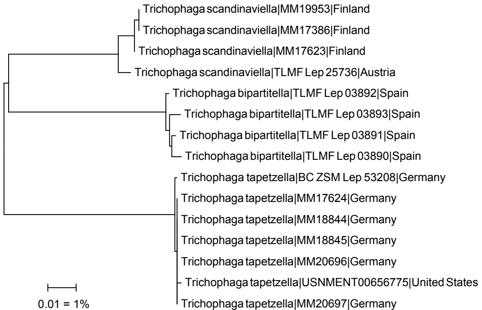
Abb. 3: Neighbour Joining tree kontinental-europäischer Trichophaga basierend auf Sequenzen des mtDNA COI-Gens (Barcodefragment 5', 658bp) (Kimura-2-Parameter, produziert mit MEGA 6; cf. TAMURA et al. 2013). / Neighbour Joining tree of continental-European Trichophaga based on sequences of the mtDNA COI gene (barcode fragment 5', 658bp) (Kimura-2-parameter distance, produced with MEGA 6, see TAMURA et al. 2013).
